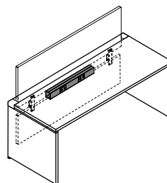
Single sided shared table up to 2 duplex outlets
