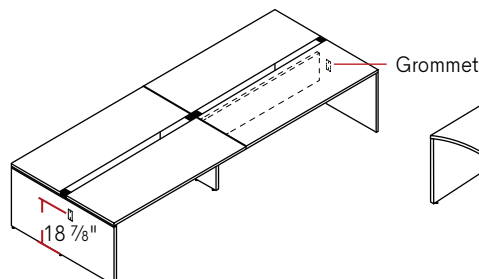
Open shared table - 2-sided - full laminate end panels
